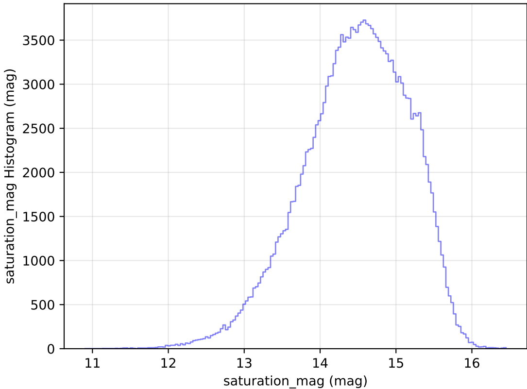
roll_pause_mjdp180_v3.4_10yrs All sky g band: saturation_mag Histogram
