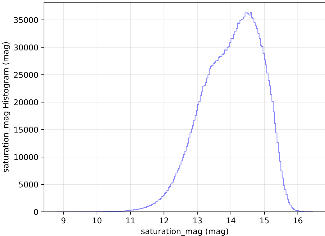
roll_pause_mjdp180_v3.4_10yrs All sky all bands: saturation_mag Histogram
