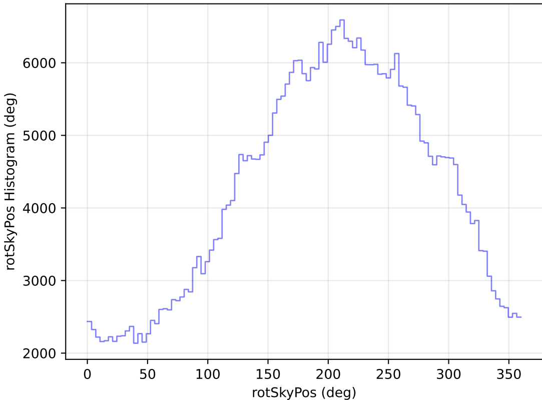
roll_pause_mjdp180_v3.4_10yrs WFD z band: rotSkyPos Histogram
