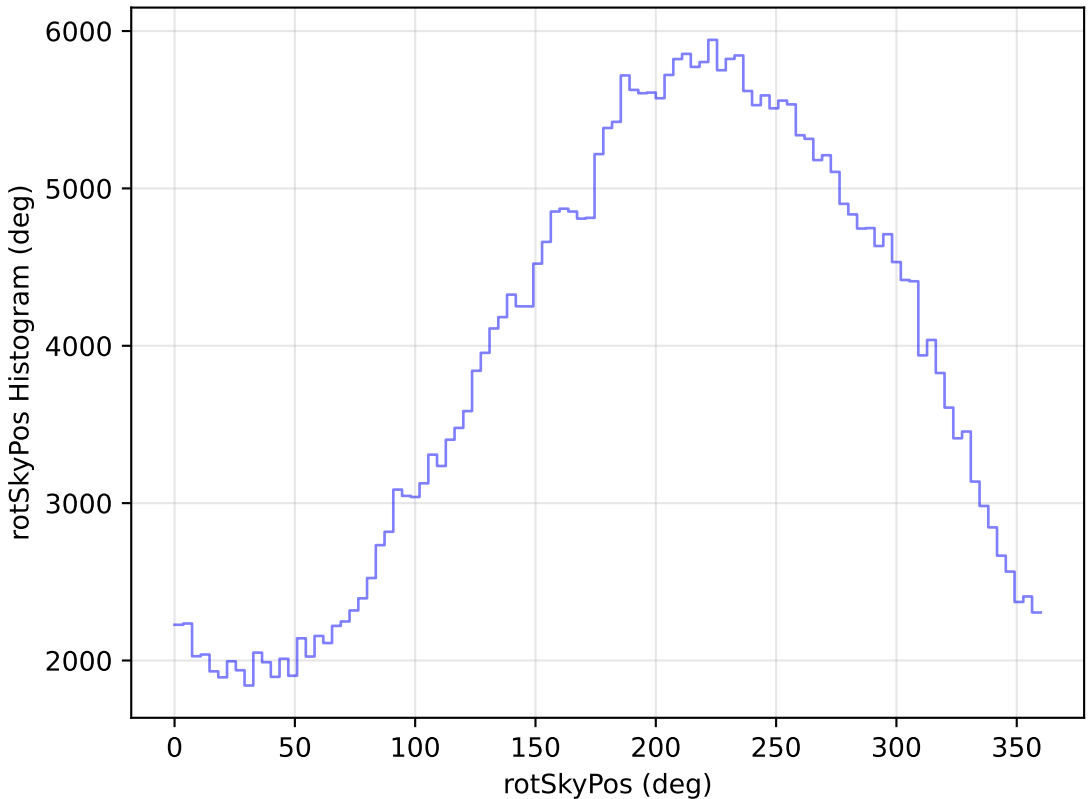
roll_pause_mjdp180_v3.4_10yrs WFD y band: rotSkyPos Histogram
