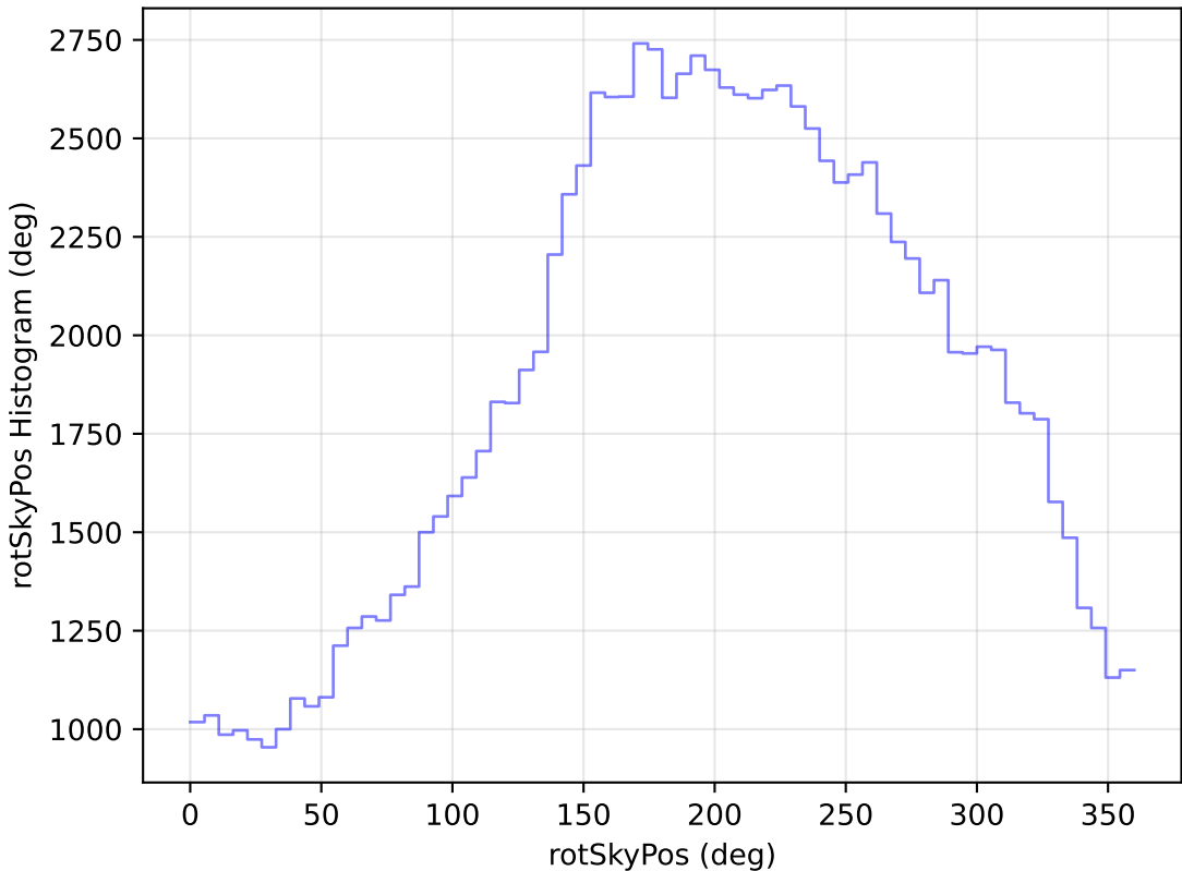
roll_pause_mjdp180_v3.4_10yrs WFD u band: rotSkyPos Histogram
