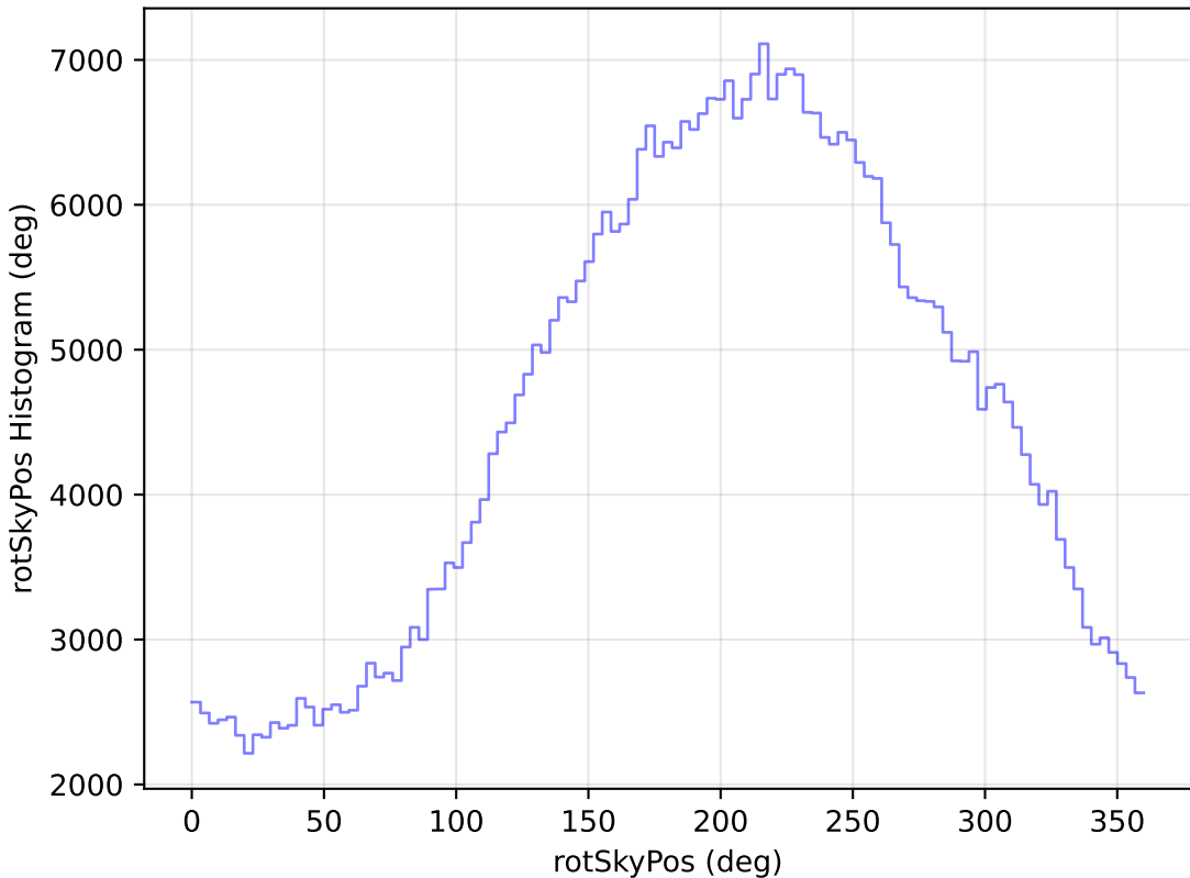
roll_pause_mjdp180_v3.4_10yrs WFD i band: rotSkyPos Histogram
