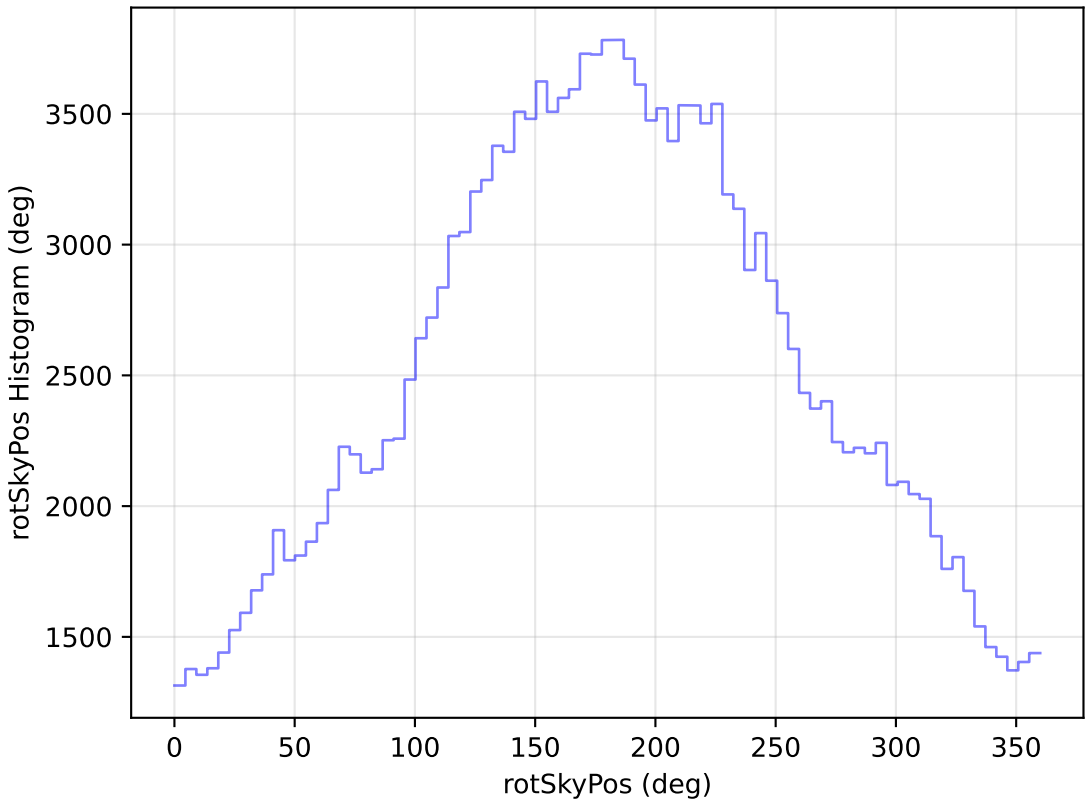
roll_pause_mjdp180_v3.4_10yrs WFD g band: rotSkyPos Histogram
