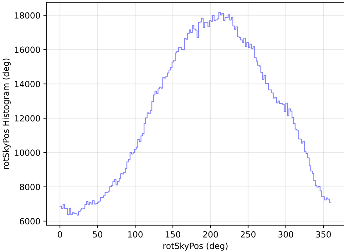
roll_pause_mjdp180_v3.4_10yrs WFD all bands: rotSkyPos Histogram
