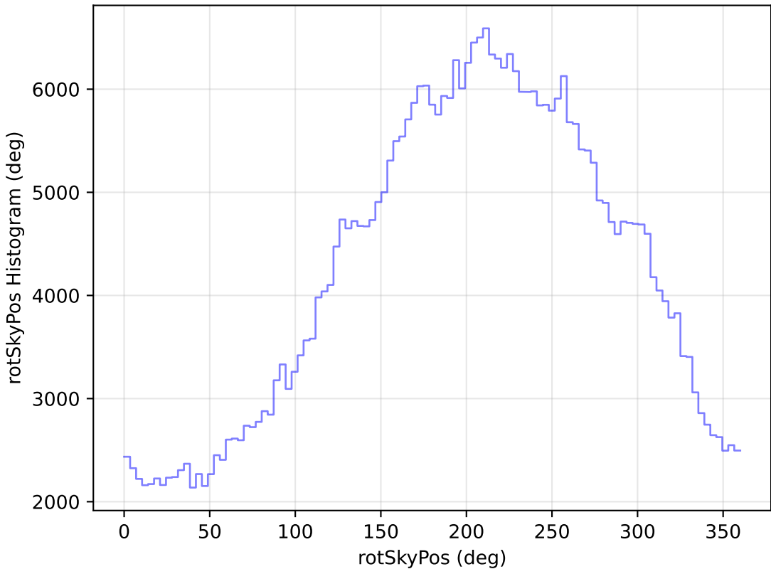
roll_pause_mjdp180_v3.4_10yrs All sky z band: rotSkyPos Histogram
