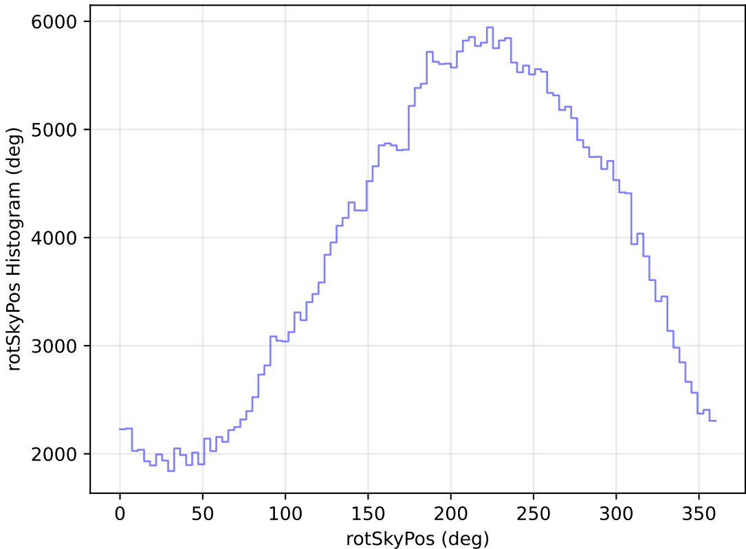
roll_pause_mjdp180_v3.4_10yrs All sky y band: rotSkyPos Histogram
