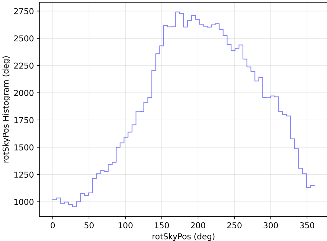
roll_pause_mjdp180_v3.4_10yrs All sky u band: rotSkyPos Histogram
