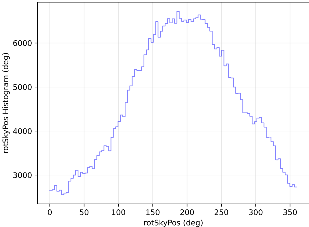
roll_pause_mjdp180_v3.4_10yrs All sky r band: rotSkyPos Histogram
