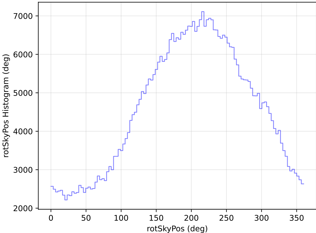
roll_pause_mjdp180_v3.4_10yrs All sky i band: rotSkyPos Histogram
