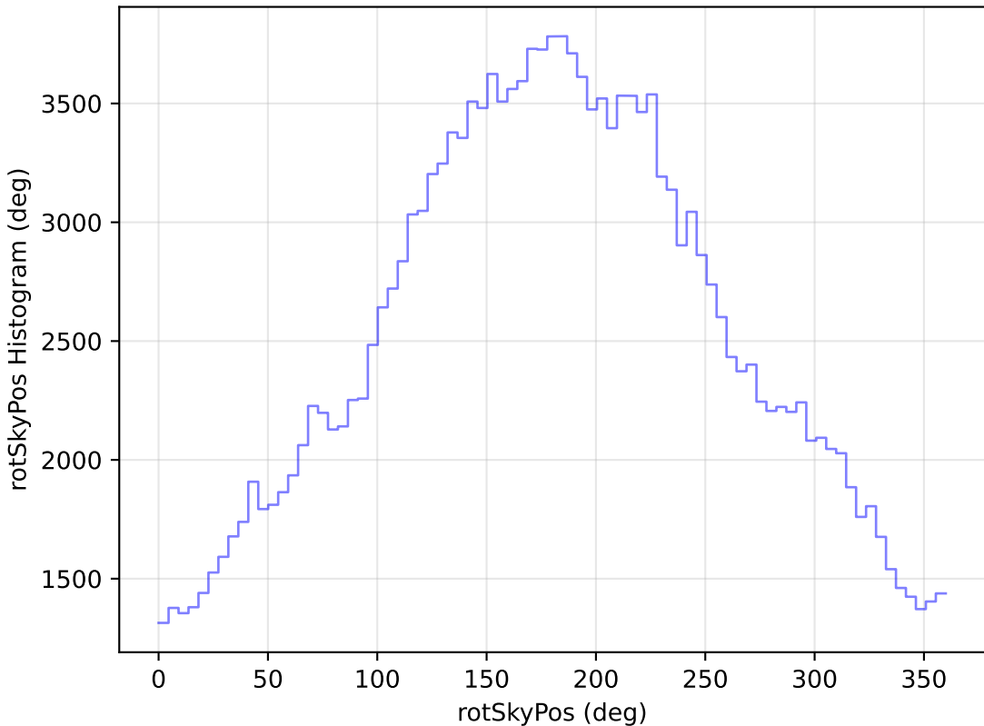
roll_pause_mjdp180_v3.4_10yrs All sky g band: rotSkyPos Histogram
