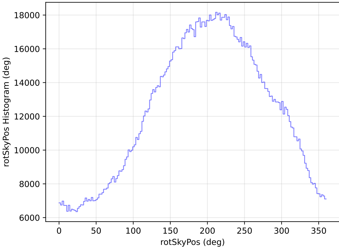
roll_pause_mjdp180_v3.4_10yrs All sky all bands: rotSkyPos Histogram
