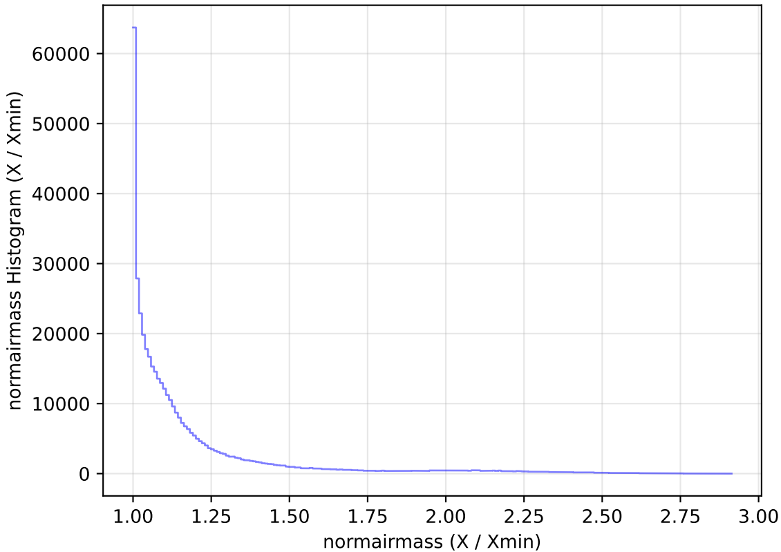
roll_pause_mjdp180_v3.4_10yrs WFD z band: normairmass Histogram
