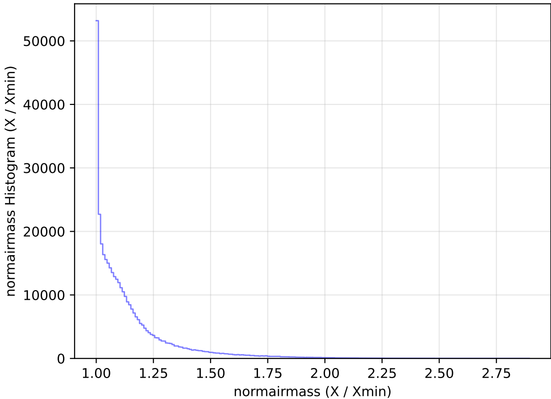
roll_pause_mjdp180_v3.4_10yrs WFD y band: normairmass Histogram
