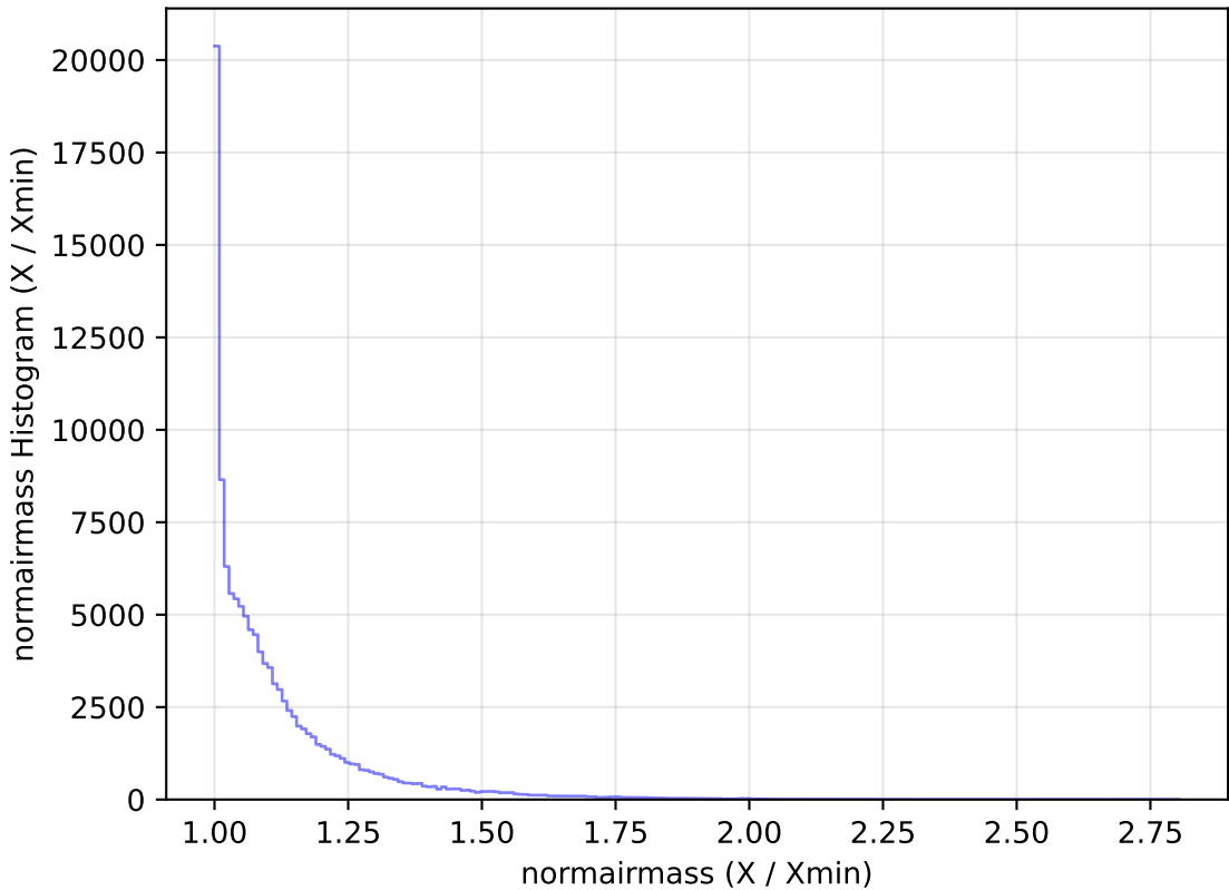
roll_pause_mjdp180_v3.4_10yrs WFD u band: normairmass Histogram
