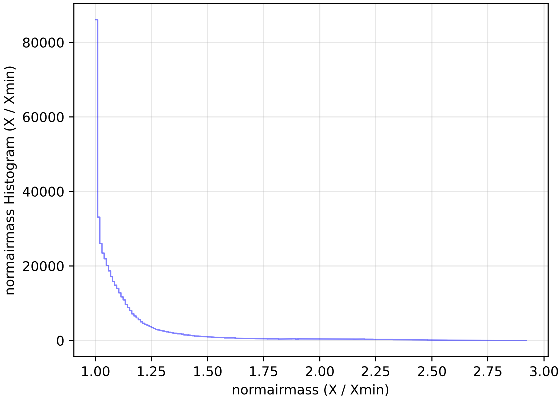
roll_pause_mjdp180_v3.4_10yrs WFD i band: normairmass Histogram
