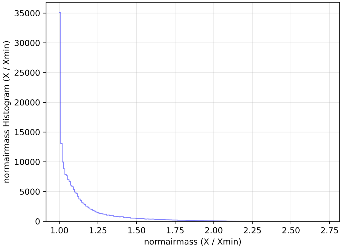
roll_pause_mjdp180_v3.4_10yrs WFD g band: normairmass Histogram
