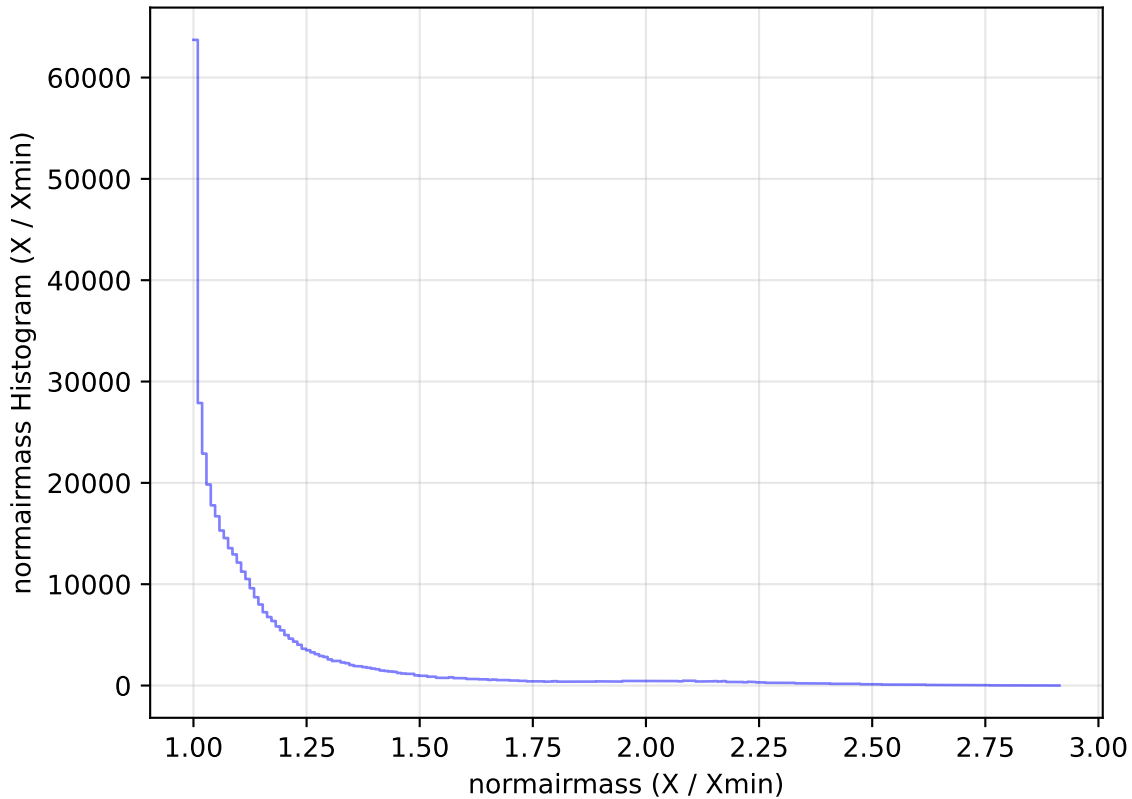
roll_pause_mjdp180_v3.4_10yrs All sky z band: normairmass Histogram
