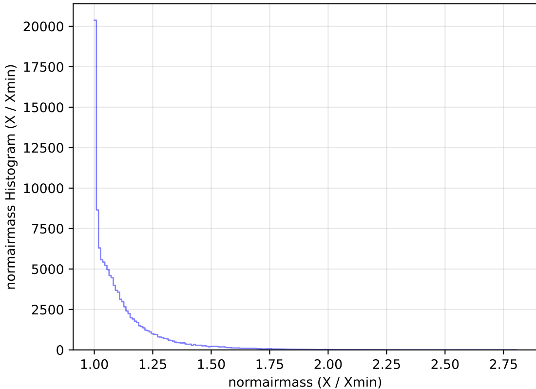
roll_pause_mjdp180_v3.4_10yrs All sky u band: normairmass Histogram
