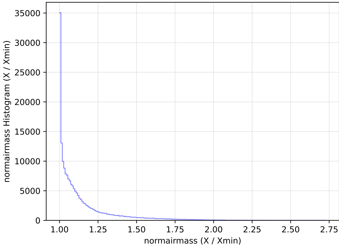
roll_pause_mjdp180_v3.4_10yrs All sky g band: normairmass Histogram
