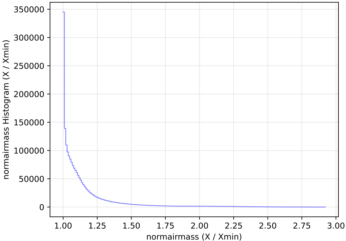
roll_pause_mjdp180_v3.4_10yrs All sky all bands: normairmass Histogram
