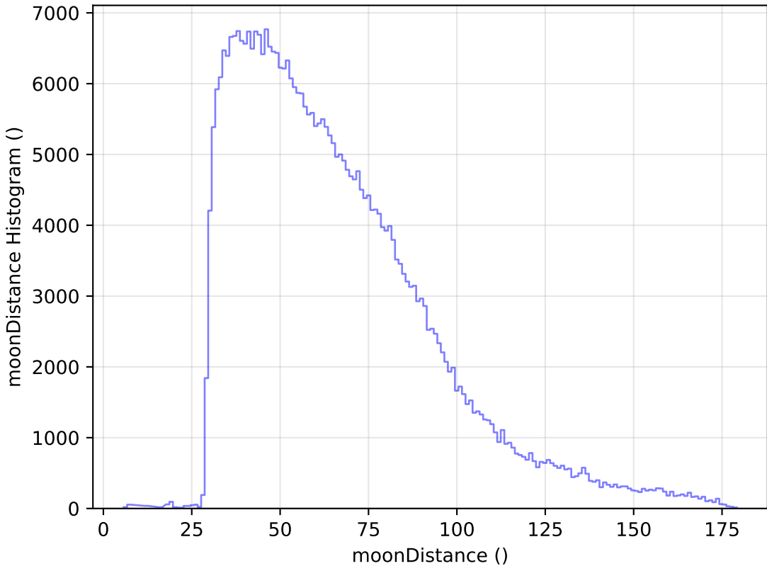
roll_pause_mjdp180_v3.4_10yrs WFD y band: moonDistance Histogram
