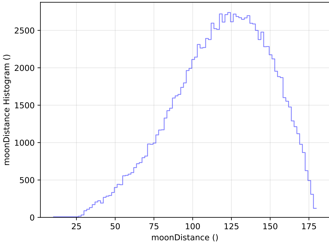
roll_pause_mjdp180_v3.4_10yrs WFD u band: moonDistance Histogram
