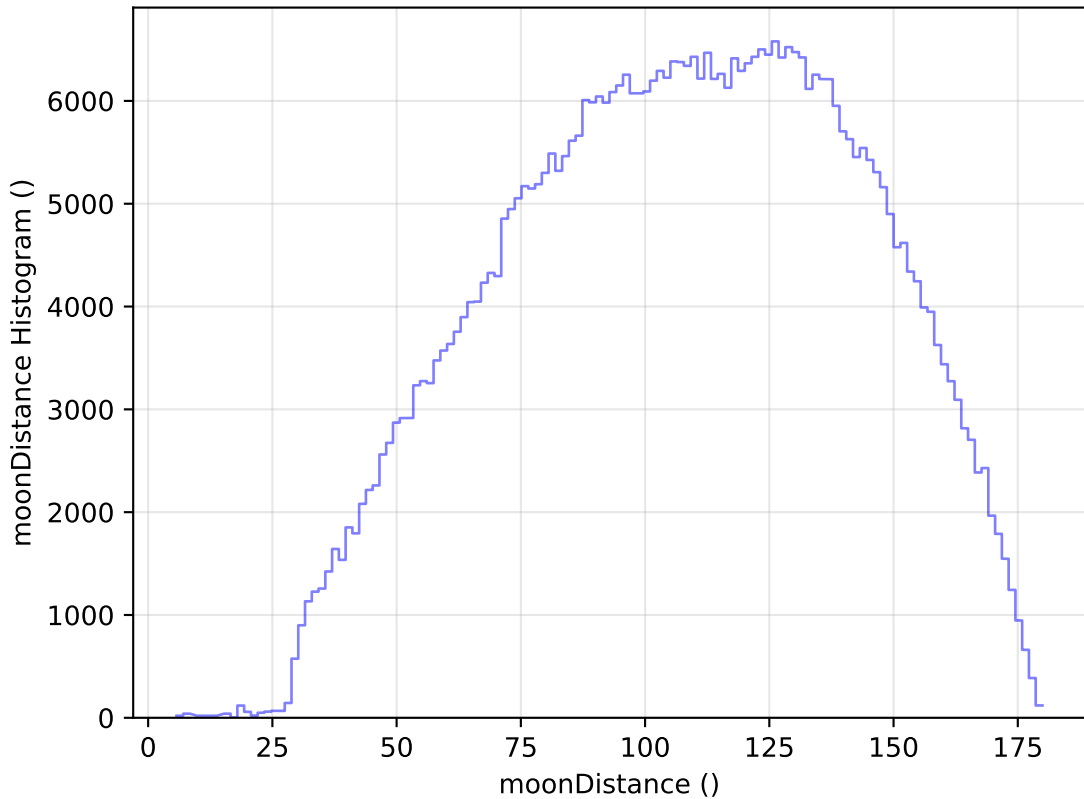
roll_pause_mjdp180_v3.4_10yrs WFD r band: moonDistance Histogram
