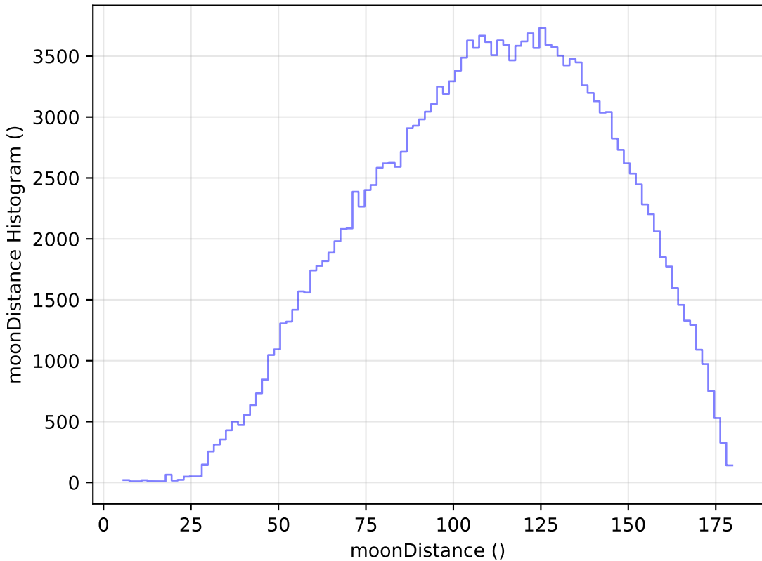
roll_pause_mjdp180_v3.4_10yrs WFD g band: moonDistance Histogram
