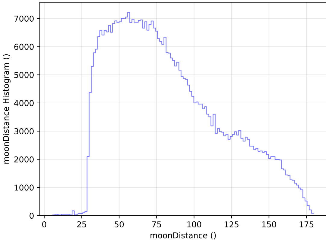
roll_pause_mjdp180_v3.4_10yrs All sky z band: moonDistance Histogram
