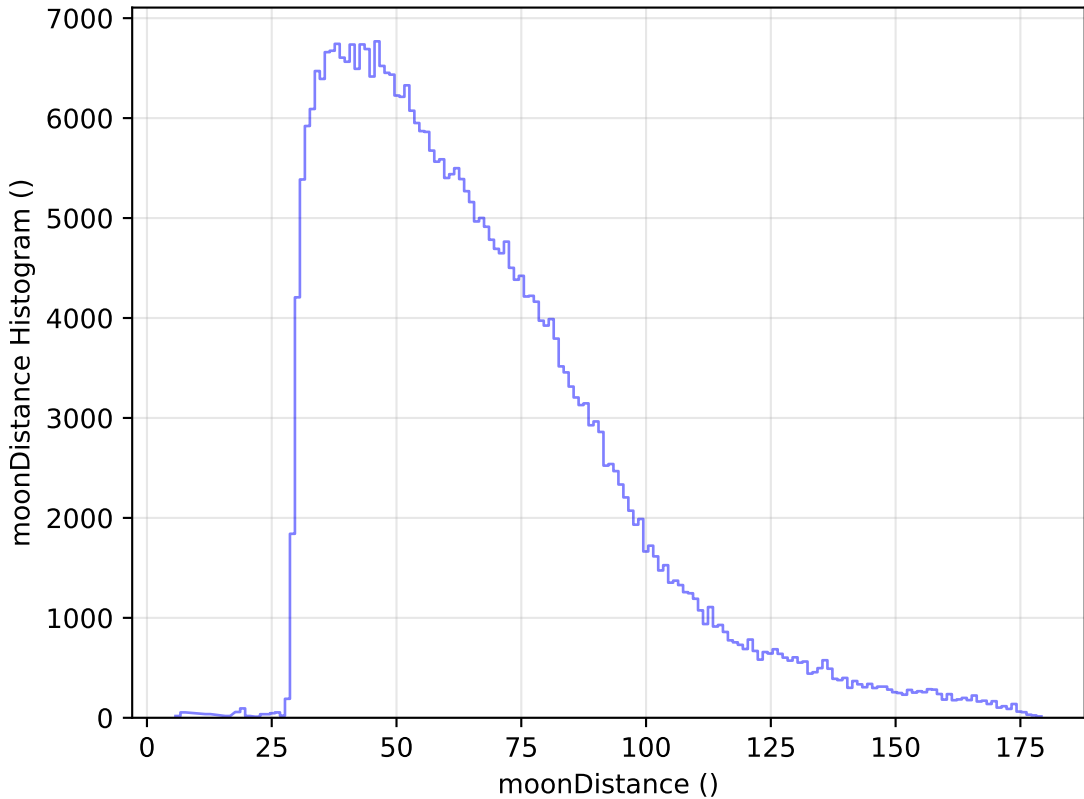
roll_pause_mjdp180_v3.4_10yrs All sky y band: moonDistance Histogram
