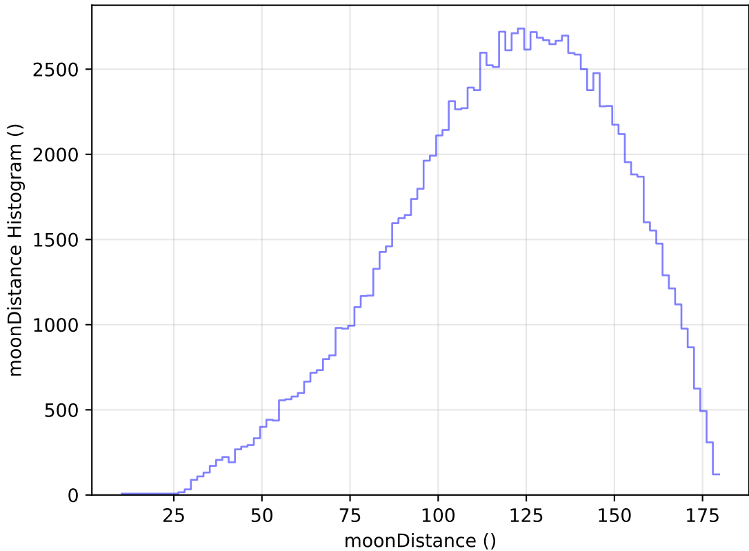
roll_pause_mjdp180_v3.4_10yrs All sky u band: moonDistance Histogram
