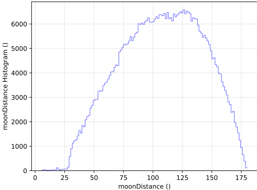
roll_pause_mjdp180_v3.4_10yrs All sky r band: moonDistance Histogram
