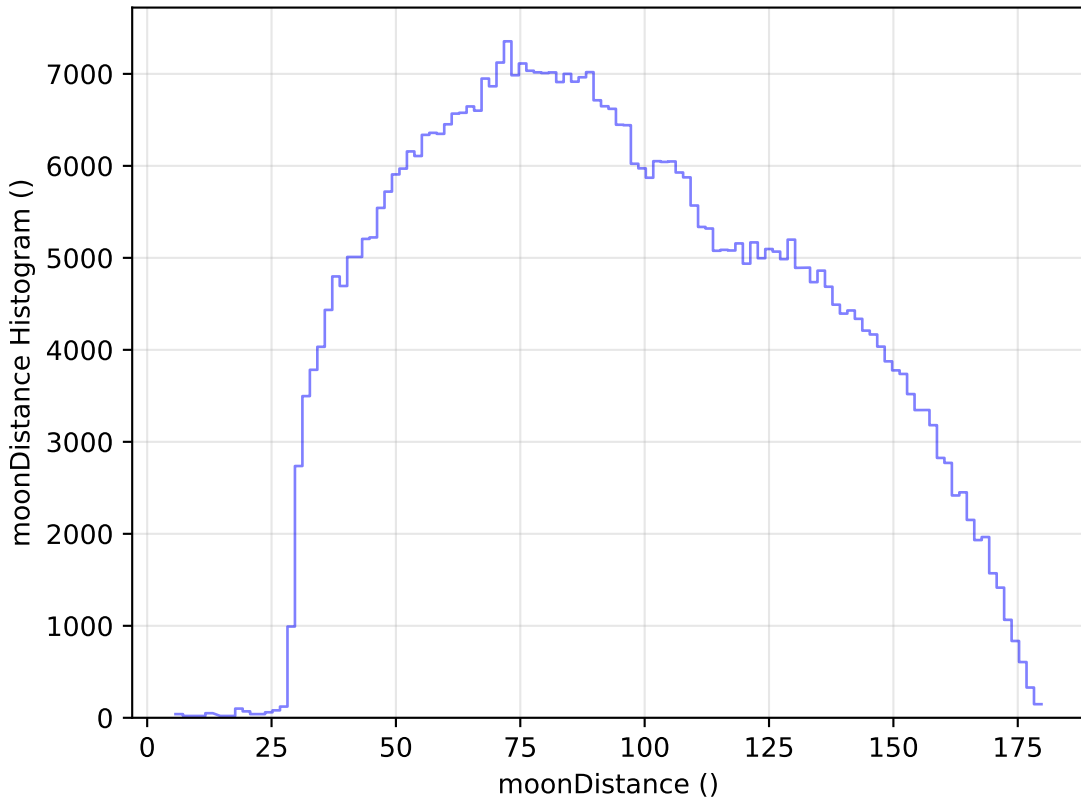
roll_pause_mjdp180_v3.4_10yrs All sky i band: moonDistance Histogram
