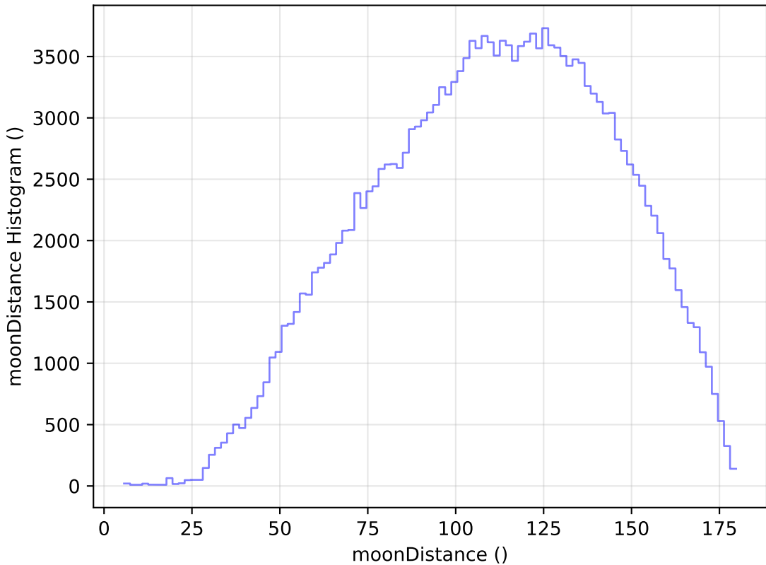
roll_pause_mjdp180_v3.4_10yrs All sky g band: moonDistance Histogram
