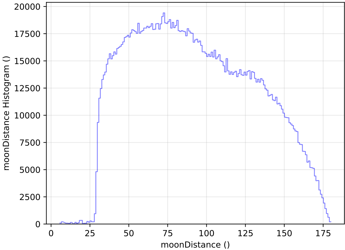
roll_pause_mjdp180_v3.4_10yrs All sky all bands: moonDistance Histogram
