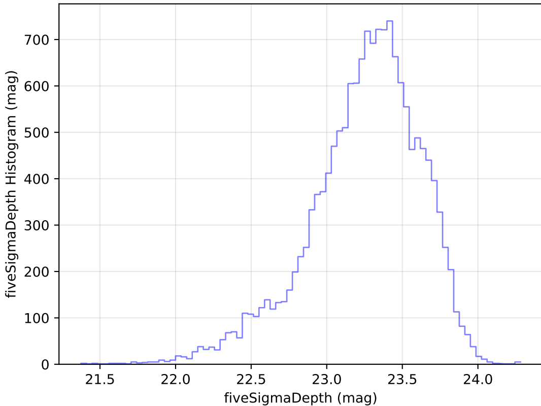
roll_pause_mjdp180_v3.4_10yrs Yr 1 u band: fiveSigmaDepth Histogram
