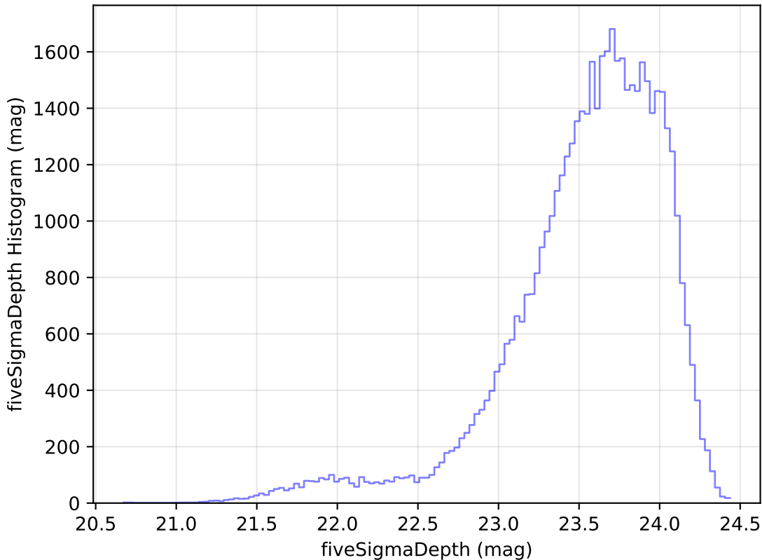
roll_pause_mjdp180_v3.4_10yrs Yr 1 i band: fiveSigmaDepth Histogram
