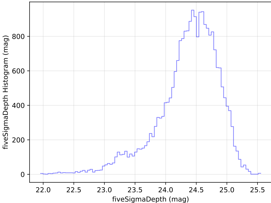
roll_pause_mjdp180_v3.4_10yrs Yr 1 g band: fiveSigmaDepth Histogram
