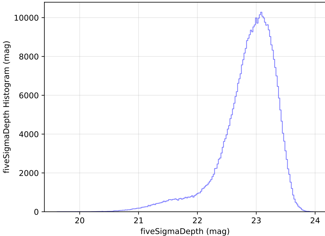
roll_pause_mjdp180_v3.4_10yrs WFD z band: fiveSigmaDepth Histogram
