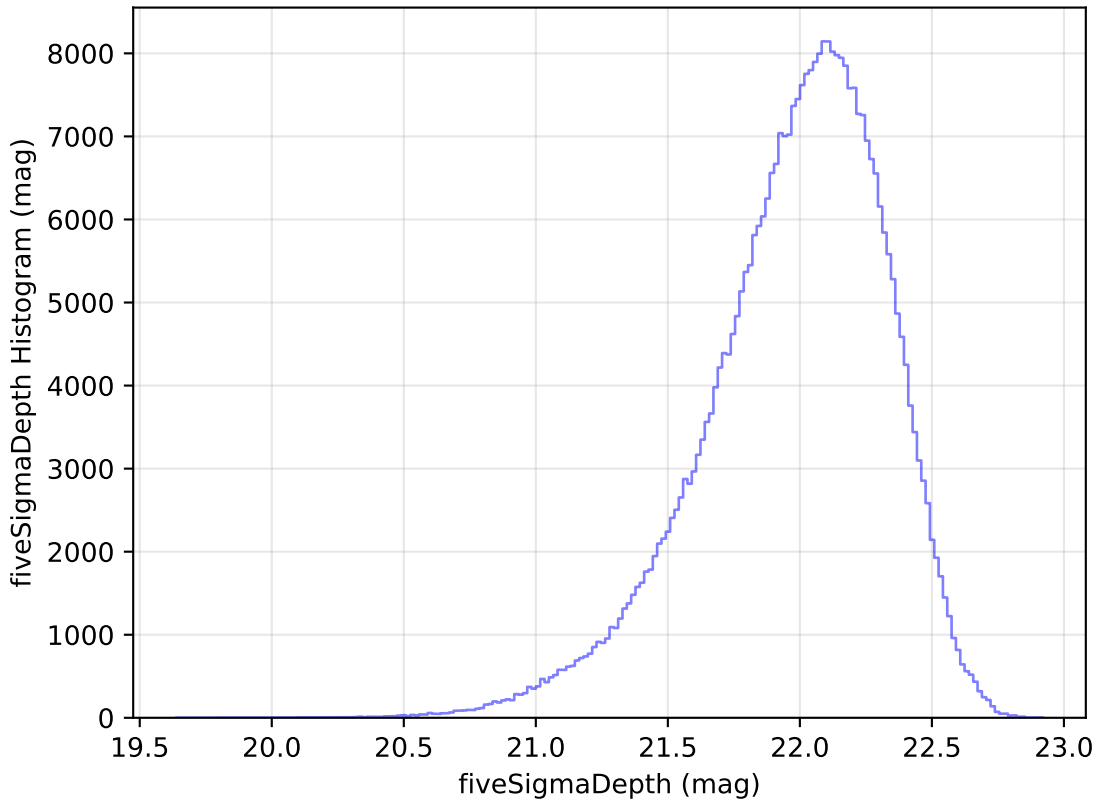
roll_pause_mjdp180_v3.4_10yrs WFD y band: fiveSigmaDepth Histogram
