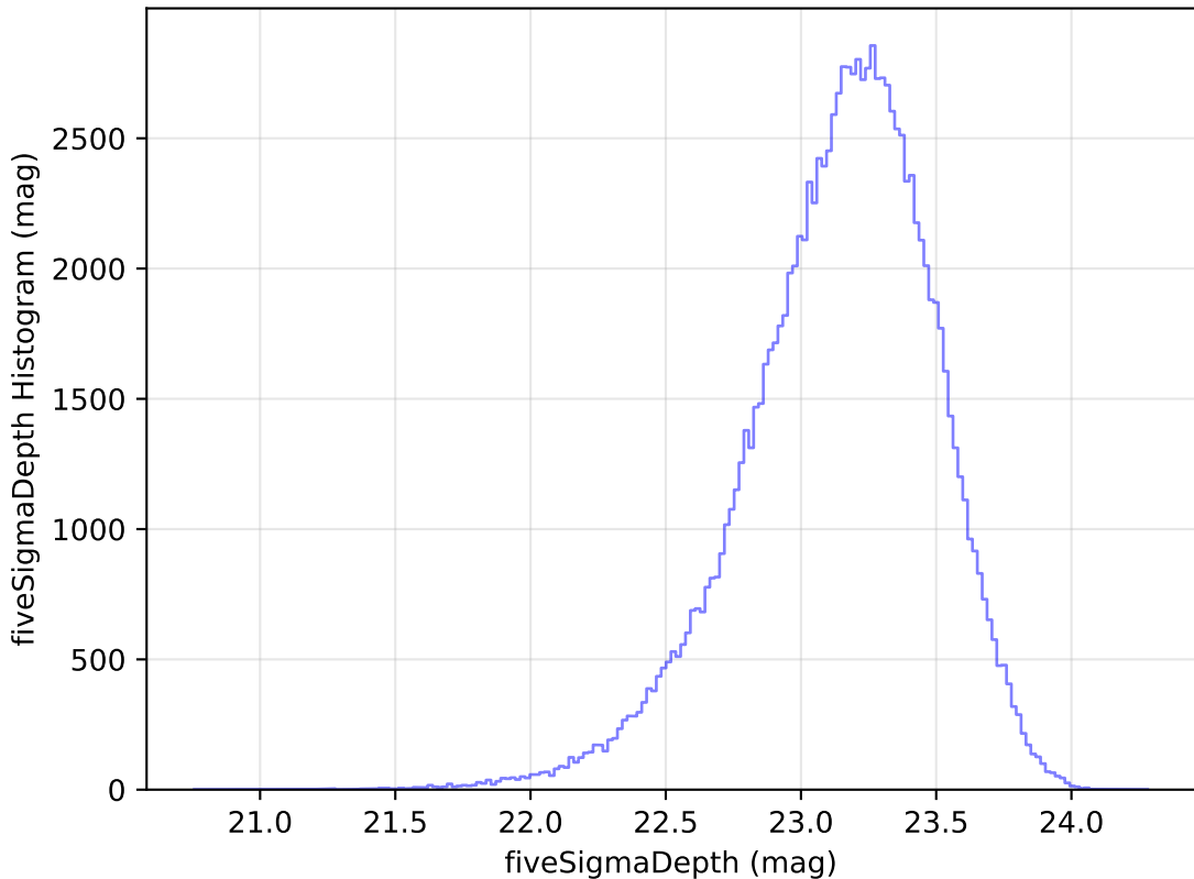
roll_pause_mjdp180_v3.4_10yrs WFD u band: fiveSigmaDepth Histogram
