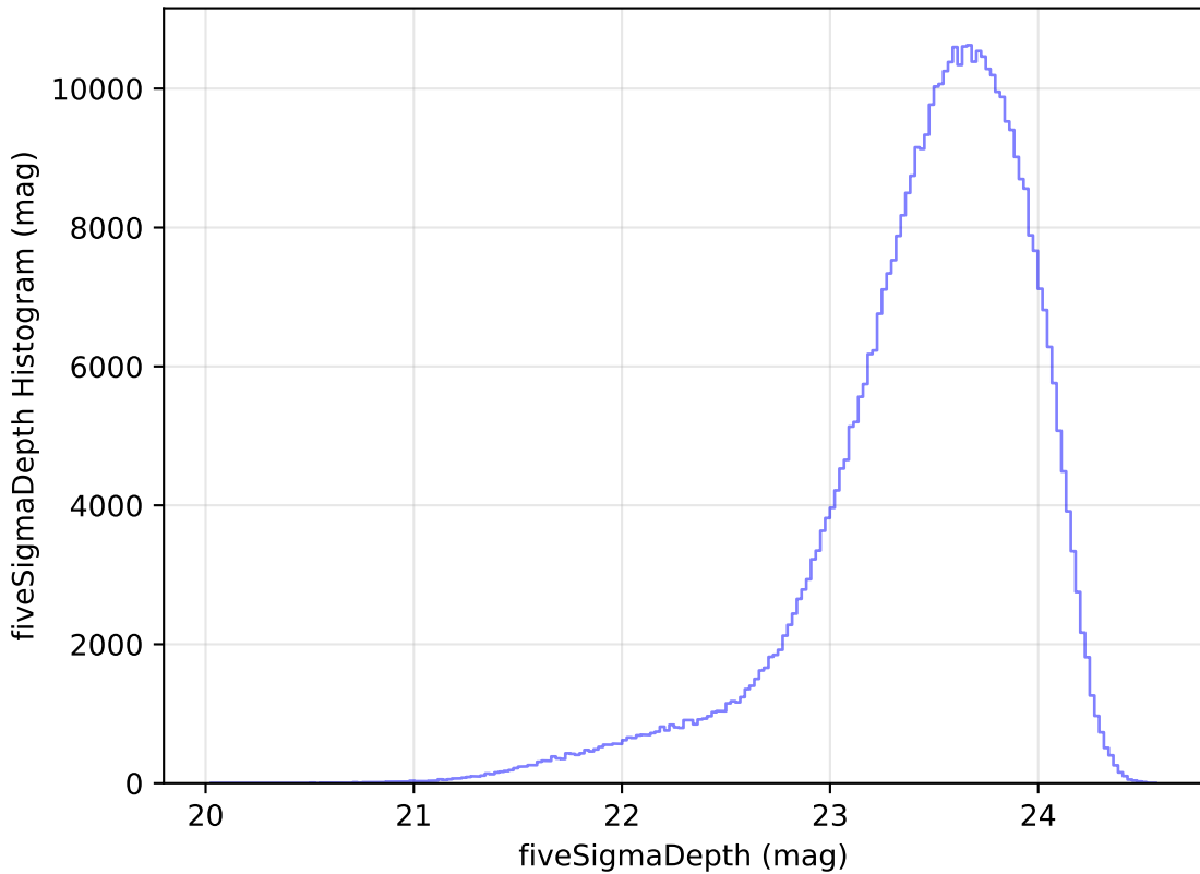
roll_pause_mjdp180_v3.4_10yrs WFD i band: fiveSigmaDepth Histogram
