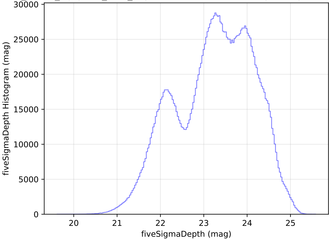
roll_pause_mjdp180_v3.4_10yrs WFD all bands: fiveSigmaDepth Histogram
