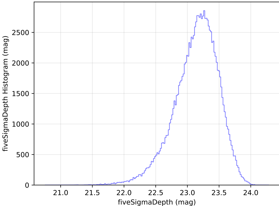
roll_pause_mjdp180_v3.4_10yrs All sky u band: fiveSigmaDepth Histogram
