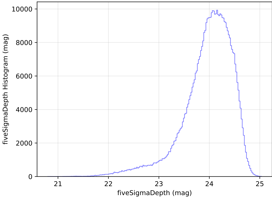
roll_pause_mjdp180_v3.4_10yrs All sky r band: fiveSigmaDepth Histogram
