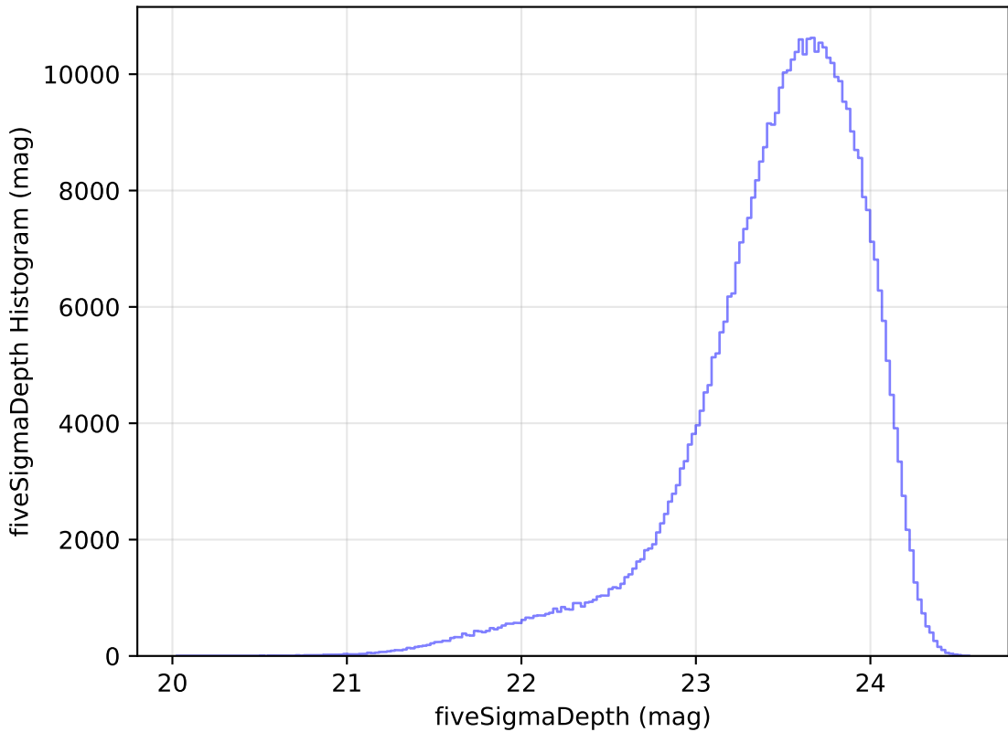
roll_pause_mjdp180_v3.4_10yrs All sky i band: fiveSigmaDepth Histogram
