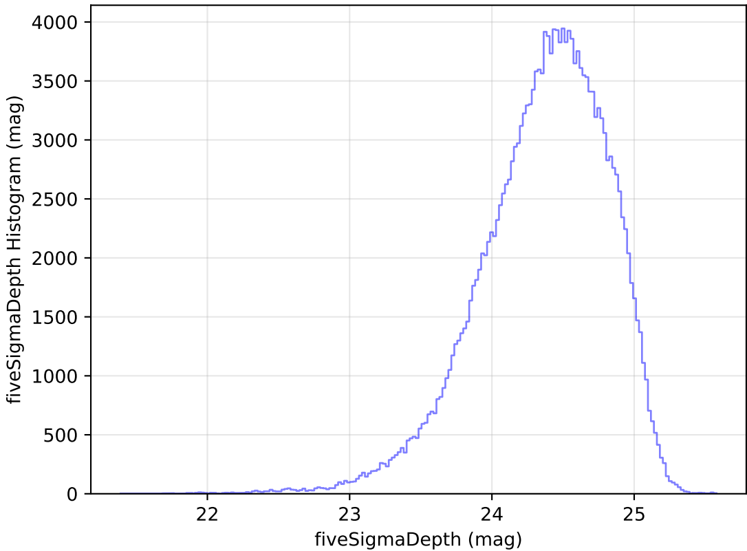
roll_pause_mjdp180_v3.4_10yrs All sky g band: fiveSigmaDepth Histogram
