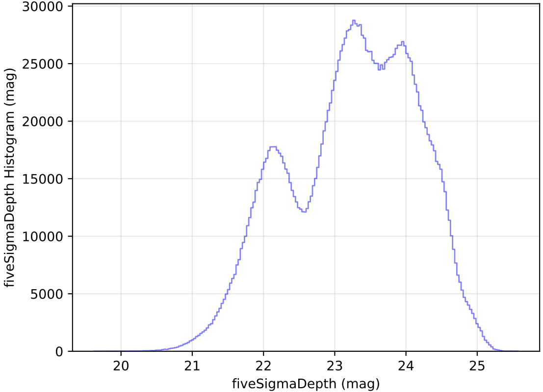
roll_pause_mjdp180_v3.4_10yrs All sky all bands: fiveSigmaDepth Histogram
