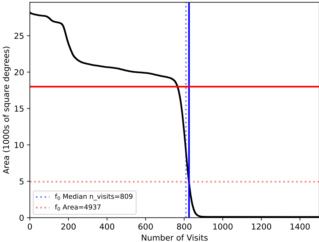
roll_pause_mjdp180_v3.4_10yrs All sky: fO
