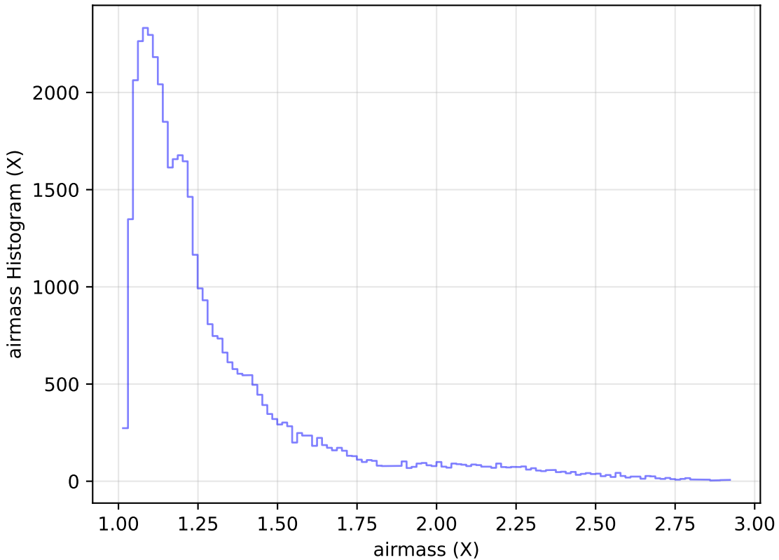
roll_pause_mjdp180_v3.4_10yrs Yr 1 z band: airmass Histogram
